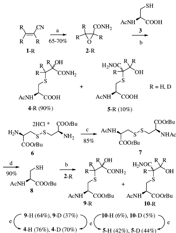
Scheme 1. Preparation of the oxidative metabolites of acrylamide (4-H, 5-H) and internal standards (4-D, 5-D) from acrylonitrile and [D 3 ]acrylonitrile, respectively: (a) 30% aq. H 2 O 2 , aq. NaOH, pH = 7.3–7.8; (b) aq. Na 2 CO 3 , MeCN, pH = 8–9; (c) Ac 2 O, pyridine, 0 °C; (d) NaBH 4 , EtOH; (e) aq. HCl, THF, 0 °C.
