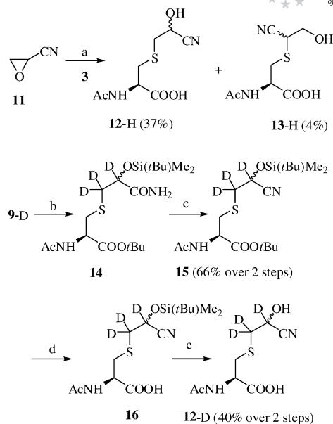
Scheme 2. Preparation of the oxidative metabolites of acrylonitrile 12-H, 13-H and the internal standard 12-D from cyanooxirane and the deuterated hydroxyamide 9-D, respectively: (a) aq. Na 2 CO 3 , MeCN, room temp.; (b) t BuMe 2 SiCl, DMF, imidazole, 5 °C, 4 d; (c) (CF 3 CO) 2 O, pyridine (2 equiv.), CH 2 Cl 2 , room temp., 16 h; (d) Et 3 SiH, TFA, CH 2 Cl 2 , 5 °C, 2 d; room temp. 1 d; (e) 51% aq. HF, MeCN, 2 h, room temp.
