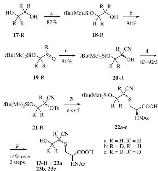
Scheme 3. Total synthesis of the oxidative metabolites of acrylonitrile 1-H(D) in the unlabelled ( 13-H ) and labelled form ( 23b-c ): (a) NaH, THF; t BuMe 2 SiCl; (b) (COCl) 2 , DMSO, –78 °C; Et 3 N, room temp.; (c) Na 2 S 2 O 5 , KCN, aq. MeOH; (d) p -MeC 6 H 4 SO 2 Cl (TsCl), pyridine; (e) MeOH/(f) [D]MeOH, Et 3 N, 40 °C 36 h; (g) 4 M HCl in dioxane.
